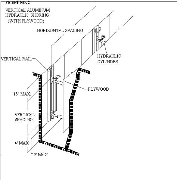
Vertical aluminum hydraulic shoring (with plywood)
