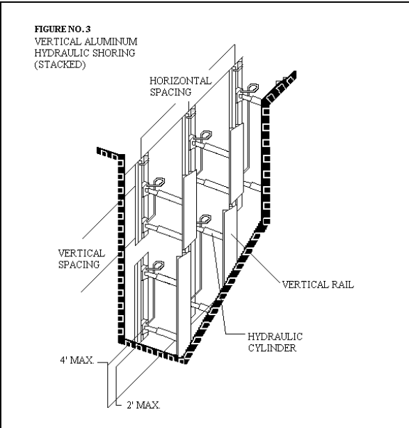
Vertical aluminum hydraulic shoring (stacked)
